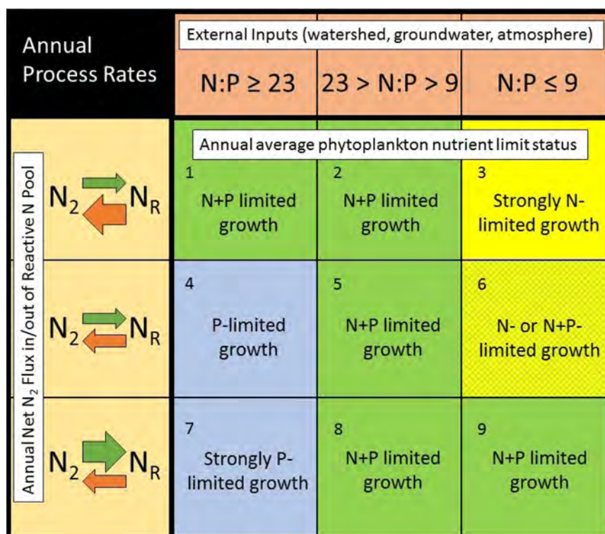
Figure 5. Conceptual model showing that the interaction between external N and P inputs and the net flux of N_2 gas into and out of the reactive N pool of lakes determines whether N or P are in shortest supply relative to phytoplankton demand and indicates a possible mechanism for explaining the preponderance of N + P colimited conditions in lakes throughout the world. The stoichiometric thresholds identified in the external inputs is derived from global patterns of phytoplankton stoichiometry and strict P limitation ( N:P \geq 23 by mass), strict N limitation ( N:P \leq 9 by mass), or N+P colimitation ( 23 > N:P > 9 ) as described by Guildford and Hecky. 75 See text for explanation.
